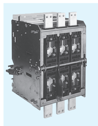
▲Front connections
