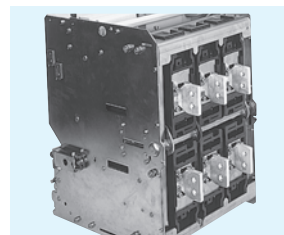
▲Vertical terminals
